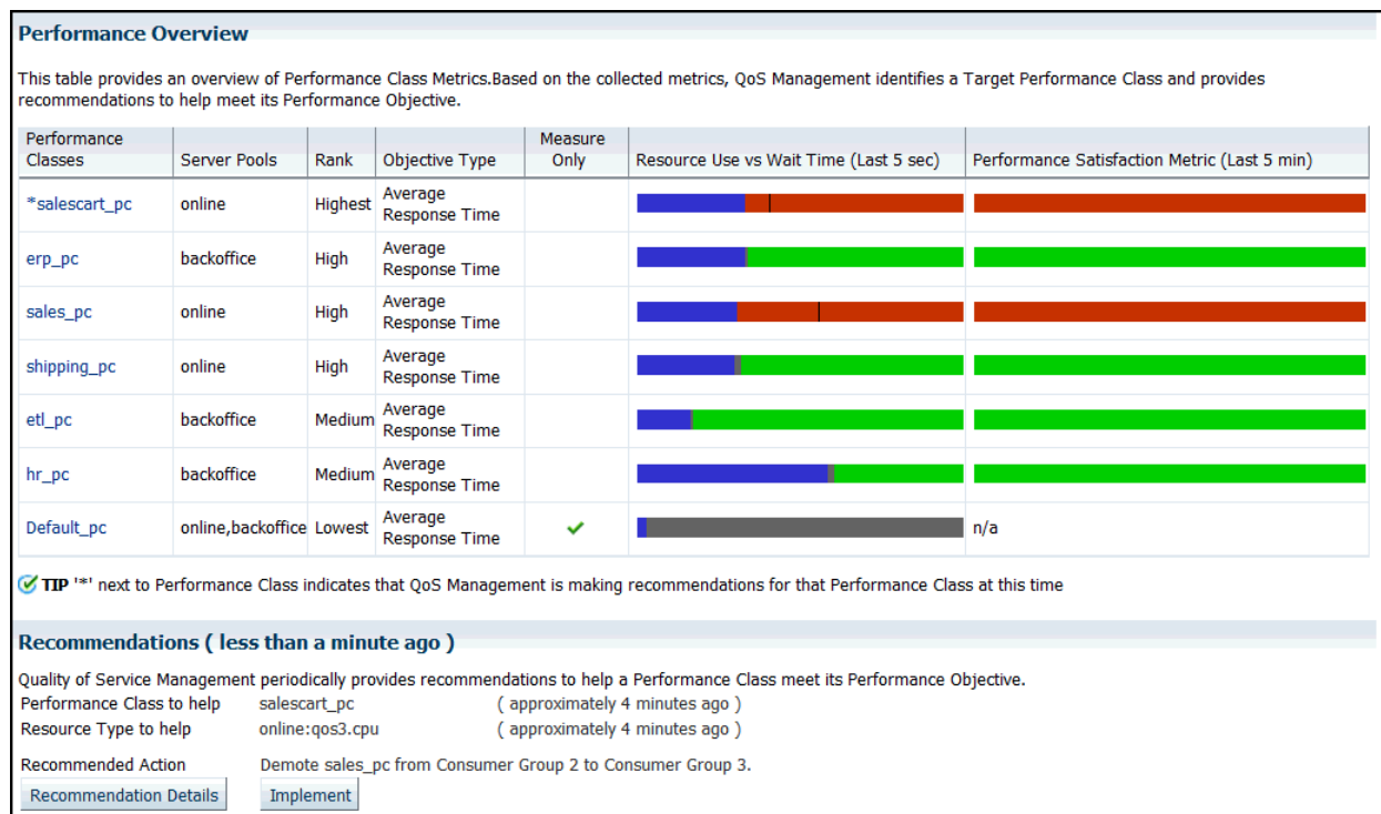
Figure 4-4 Performance Overview Page Showing Performance Classes Not Meeting Their Performance Objectives
