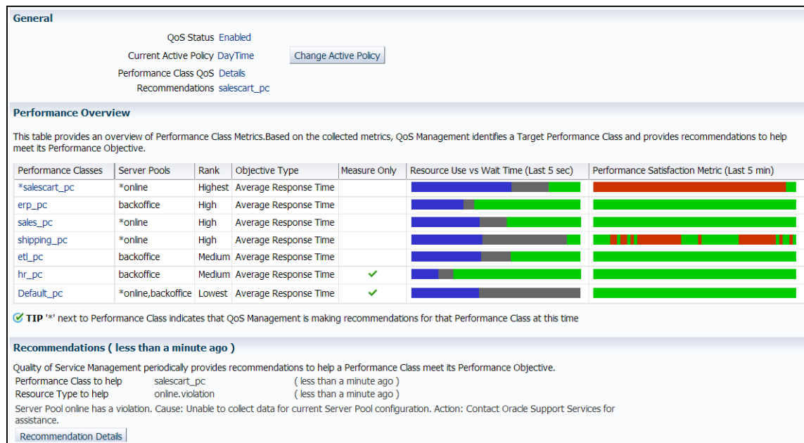
Figure 4-2 Oracle Database Quality of Service Management Dashboard
